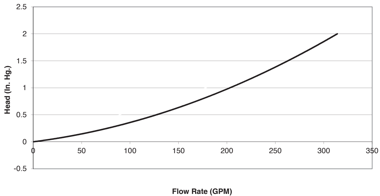
8" TRU-FLOW Head Loss Curve
